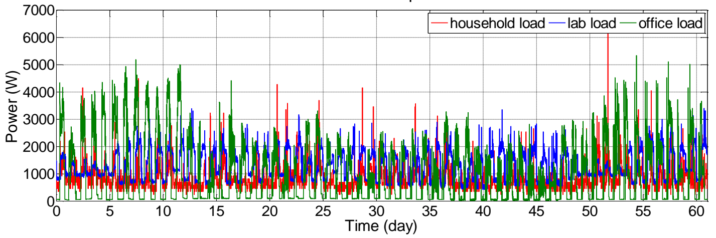
Standard load profiles
