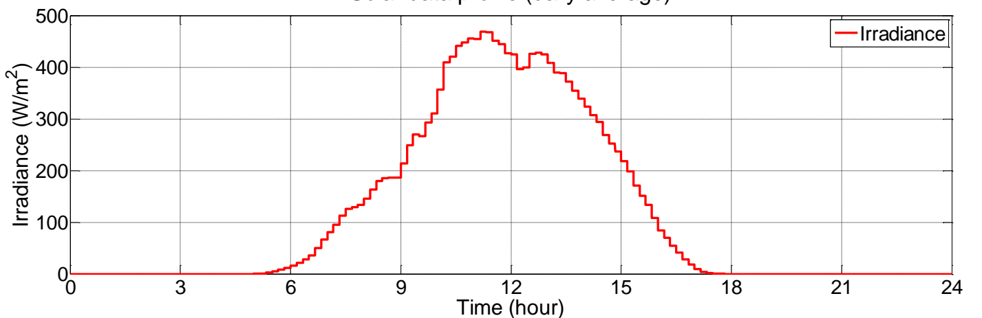
Solar data profile (daily average)
